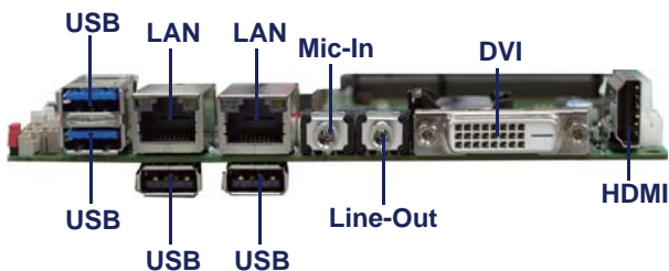
31847A / 31847C Rear I/O
